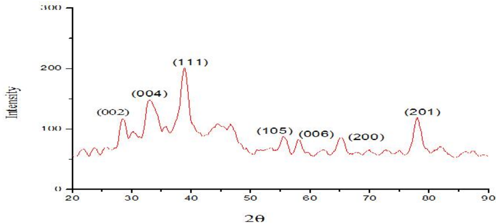
Figure 4- XRD pattern of silver nanoparticles.
