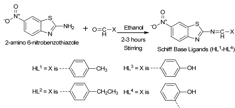
Fig. 1. Scheme of the synthesis of ligands HL 1 -HL 4 .
