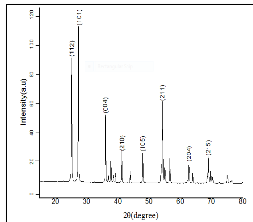
Fig-3: XRD pattern of TiO_2 nanoparticles calcinated at 500^\circ C .
