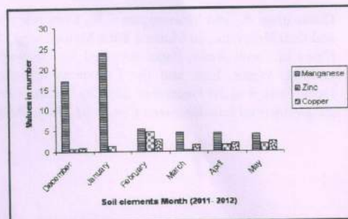
Figure-4 Soil Manganese, Zinc and Copper values from Mangulam Wetlands during December 2011 to May 2012
