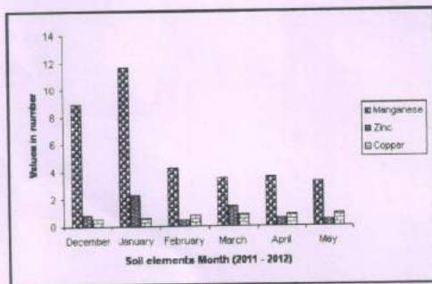
Figure-2 Soil Manganese, Zinc and Copper values from Sengulam Wetland during December 2011 to May 2012
