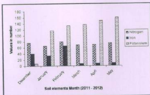
Figure-3 Soil Nitrogen, Iron and Potassium values from Mangulam Wetland during December 2011 to May 2012
