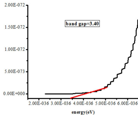
Fig.4 (\alpha hv)^2 vs h\nu curve
