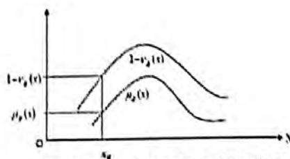
Figure 1. Intuitionistic fuzzy set explanation of real number R
