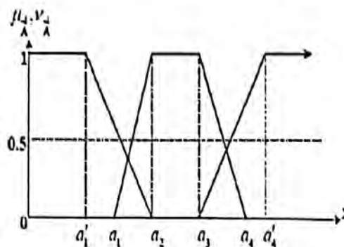
Figure 2: Membership and non-membership function of TrIFN
