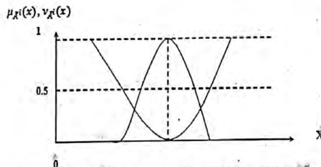
Fig. 2 Membership and non membership functions of \tilde{A}^i
