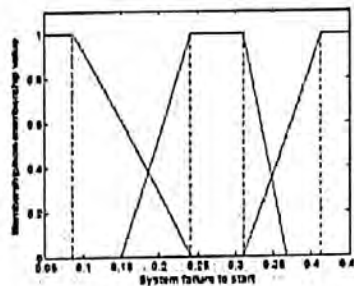
TrIFN representing the system failure to start an automobile
