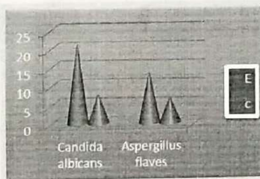
Figure 5: Antifungal activities of crude chloroform extract methanol extract of M. citrifolia against pathogens.
