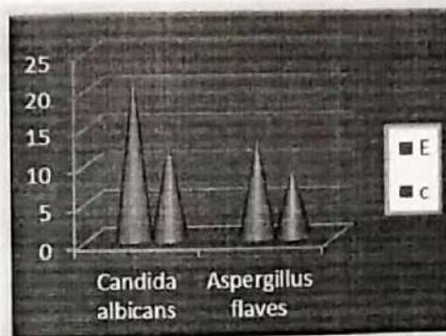
Figure 3: Antifungal activities of crude methanol extract ethyl acetate extract of M. citrifolia against pathogens.
