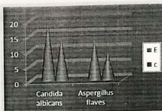
Figure 4: Antifungal activities of crude of M. citrifolia against pathogens.
