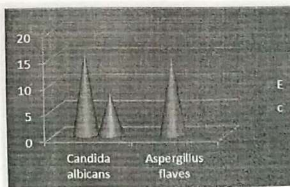
Figure 2: Antifungal activities of crude of A. indicum against pathogens.
